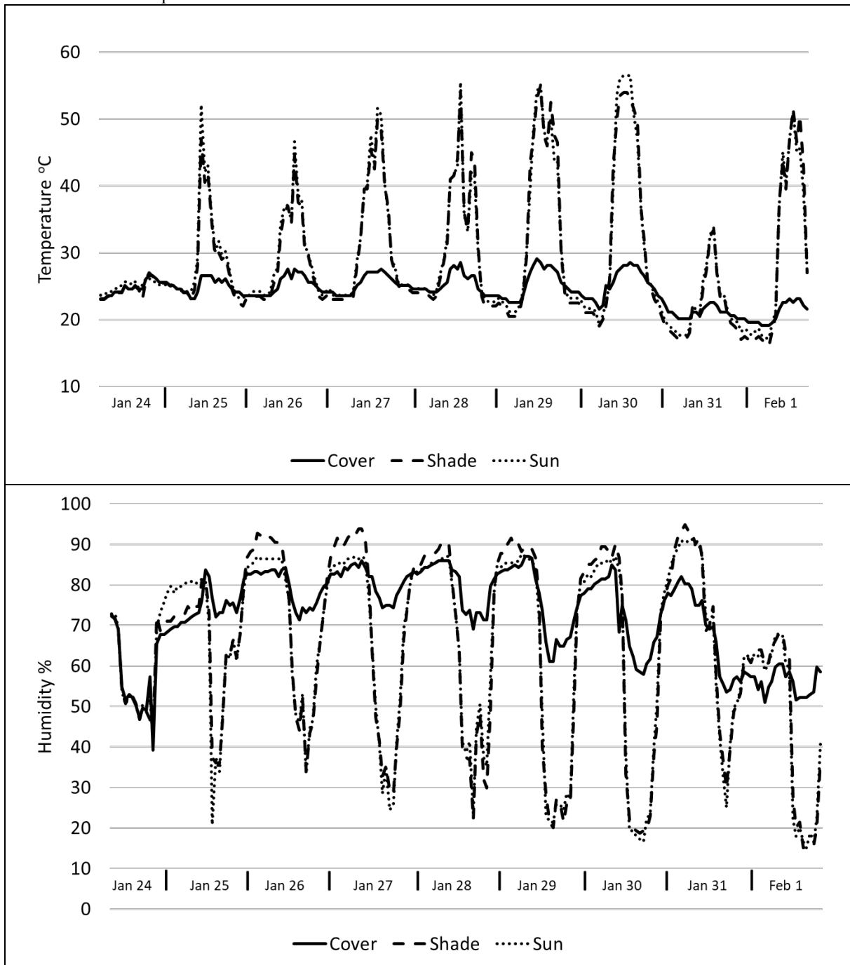
Figure 3. Temperature (a) and humidity (b) profiles in the tubs over the study period as recorded by Thermodata DS1921G i-Button probes.
