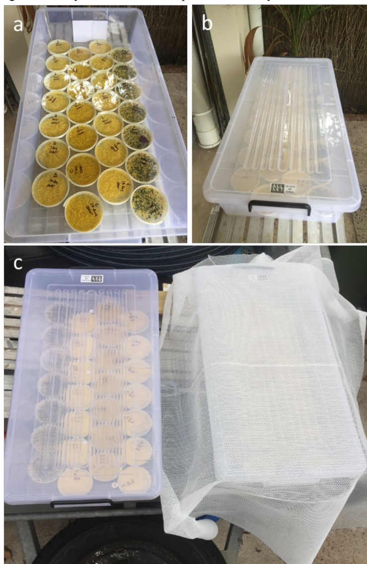
Figure 1: Exposure scenario for ant bait a. Sheltered tub shown without lid b. Sheltered tub with lid in place c. Full sun and shaded tubs with lids and shade cloth in place. NB petri dishes are labelled out to 14 days of exposure but these were adjusted during to the study for a maximum exposure of 8.5 days.
